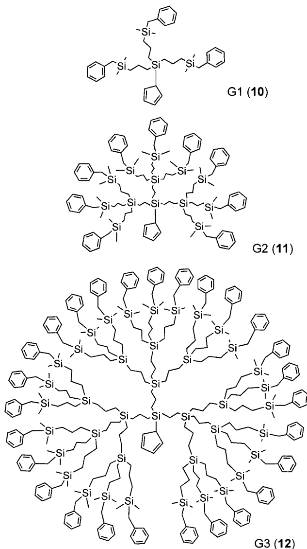
Scheme 5. Cyclopentadienes with carbosilane dendritic wedges of first ( 10 ), second ( 11 ), and third generation ( 12 ). Only the major isomers are represented.
